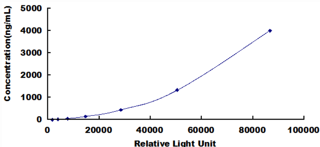
Typical Standard Curve for Antithrombin, Human CLIA.
